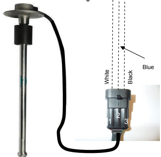
Pin 1 - Wh - Low Fuel Warning Pin 2 - Bl - Output signal Pin 3 - Bk - Negative
