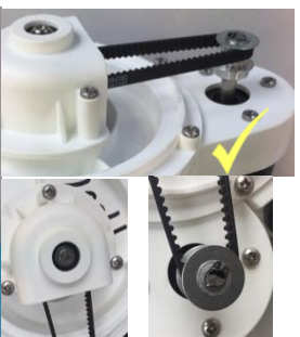
13. Replace cover and screws
