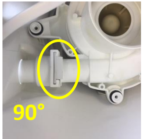
7. Turn clip 90° and remove
