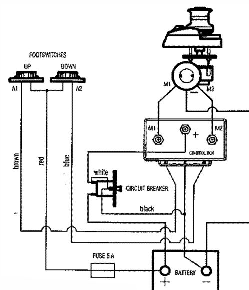
WIRING DIAGRAM - 3 TERMINALS ELECTRIC MOTOR
