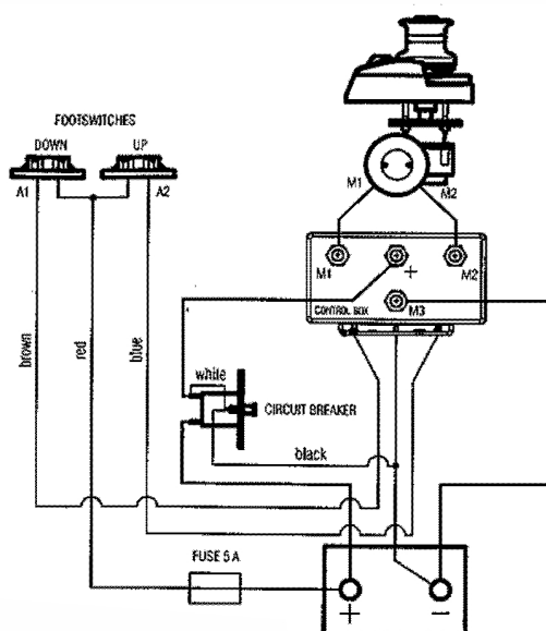
WIRING DIAGRAM - 2 TERMINALS ELECTRIC MOTOR
