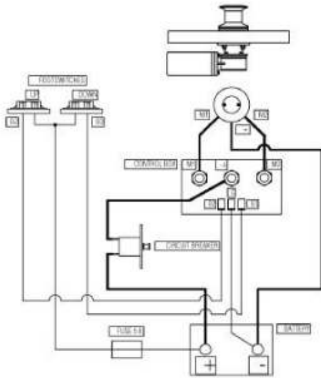
3 TERMINAL MOTORS
