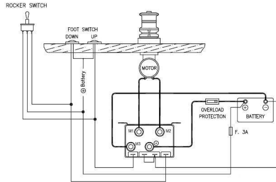
2 TERMINAL MOTORS
