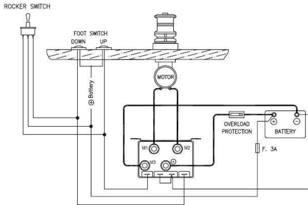
2 TERMINAL MOTORS
