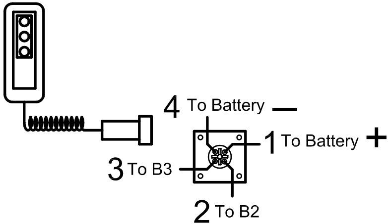
REMOTE CONTROL VEGA
