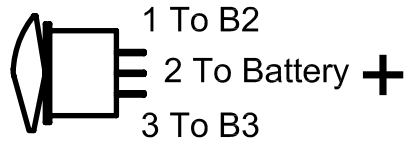
ROCKER SWITCH TYPE C
