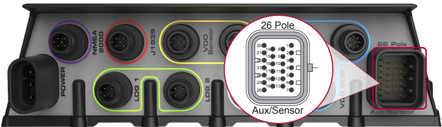
26 Pole Pinout
