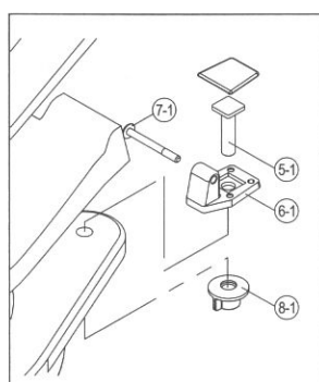
TMC-TT9924 HINGE SET FOR DELUXE SEAT ORDER NO. 504-0299024
