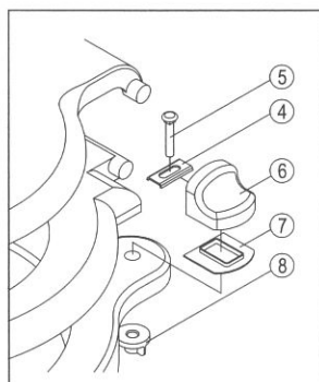
TMC-TT9923 HINGE SET FOR STANDARD SEAT ORDER NO. 504-0299023
