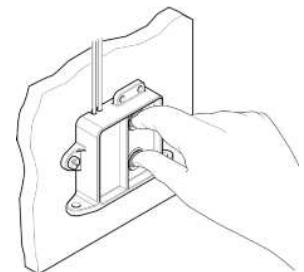
Fig 4 - Testing Switch
