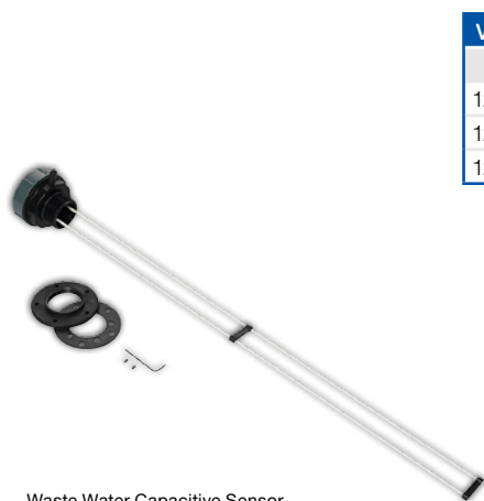
Waste Water Capacitive Sensor
